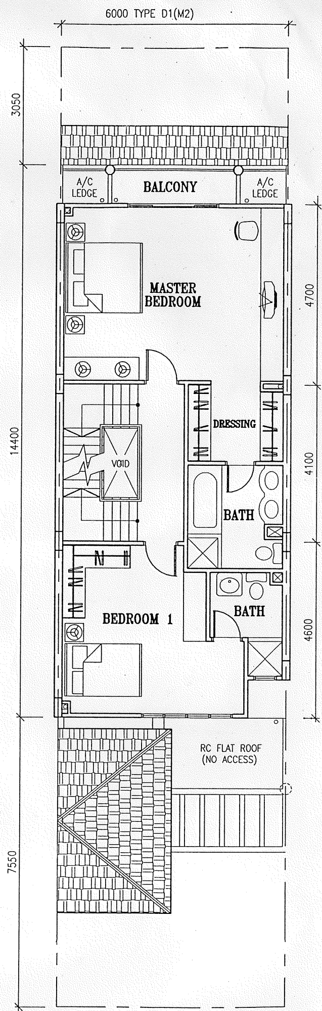
2ND STOREY PLAN TYPE D(M2)
