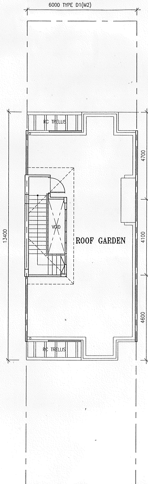
ROOF GARDEN PLAN TYPE D(M2)
