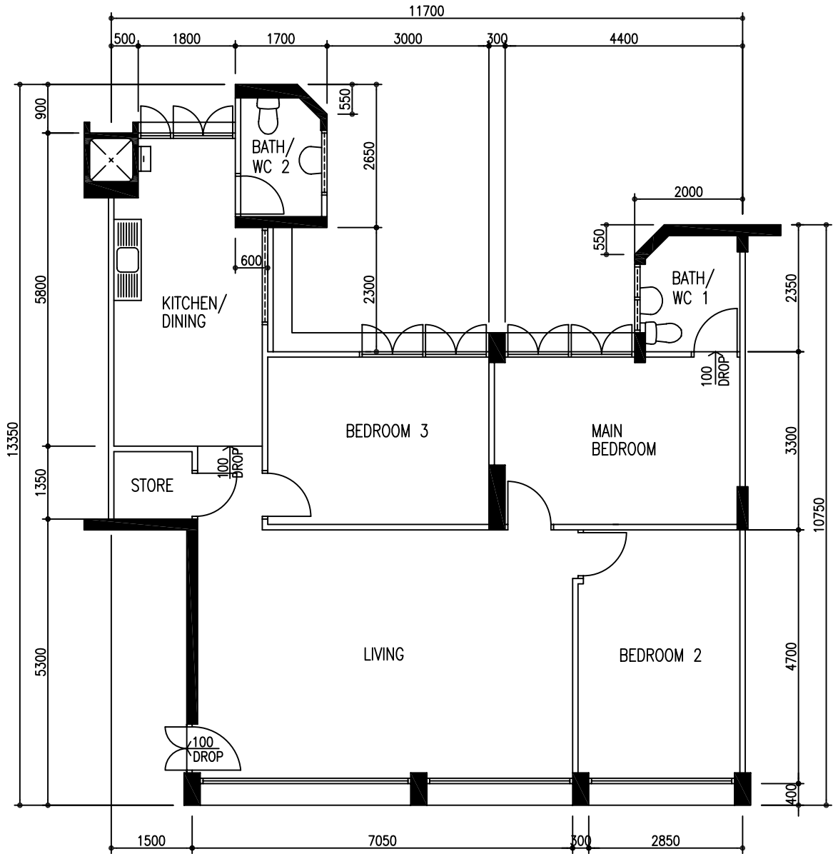
4-ROOM MODEL 'A' (STAIRS) SCALE 1:100
